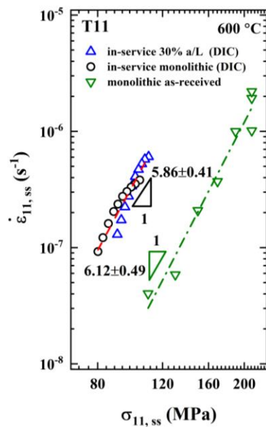
Fig. 4: Master plot showing the variation of steady-state strain rate with steady-state stress for composite (30% a/L ) and monolithic cantilevers of service-exposed T11. For comparison, steady-state creep data obtained from as-fabricated T11 monolithic cantilevers is also shown.
